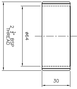
(SCALE:1:4) DETAIL-A BUSH FOR COUPLER
